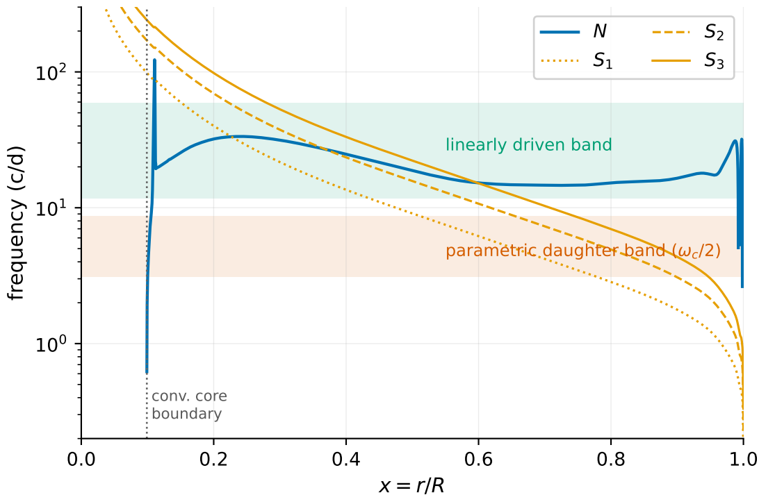
Propagation diagram, M = 1.70 M_{\odot} \delta Sct model
